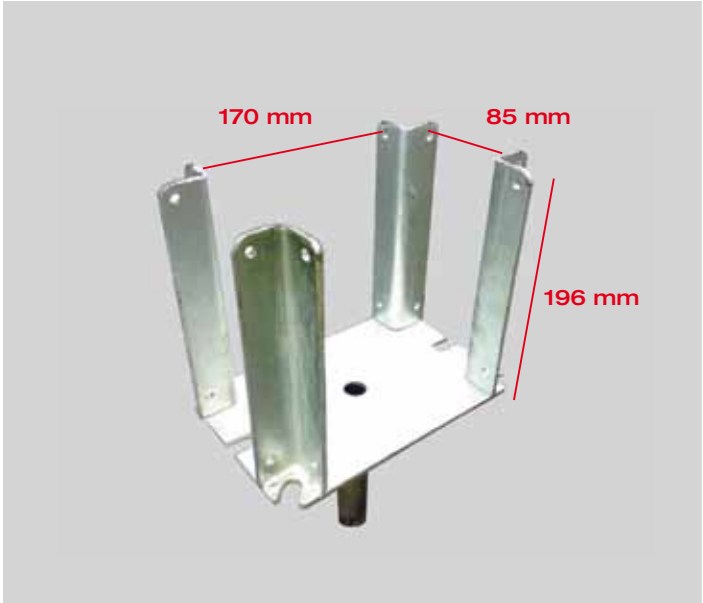
Cabezal reforzado / Reinforced head / Fourche double
